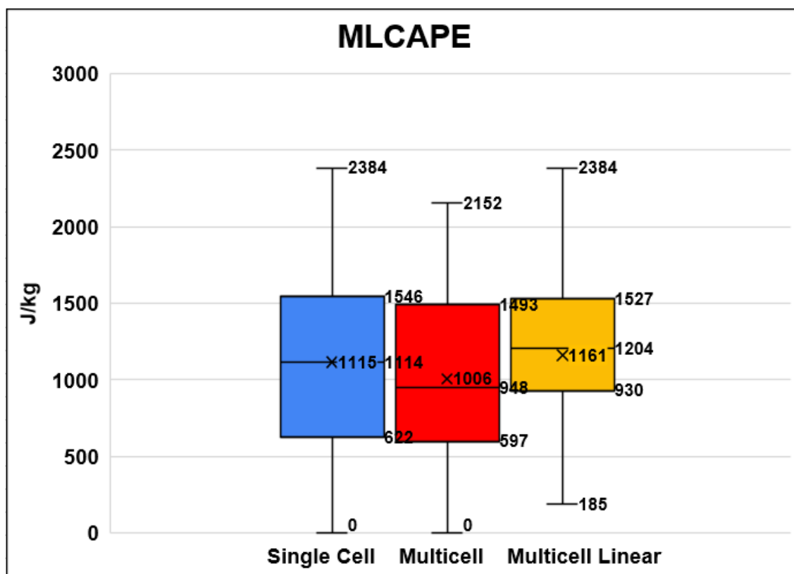
Figure 6: MLCAPE ( J\ kg^{-1} ) by storm classification type. The top and bottom of the shaded boxes denote the 75th and 25th percentile values, respectively, with the horizontal line the median and the “X” the mean. The whiskers extend upward to the 90th and downward to the 10th percentiles.
