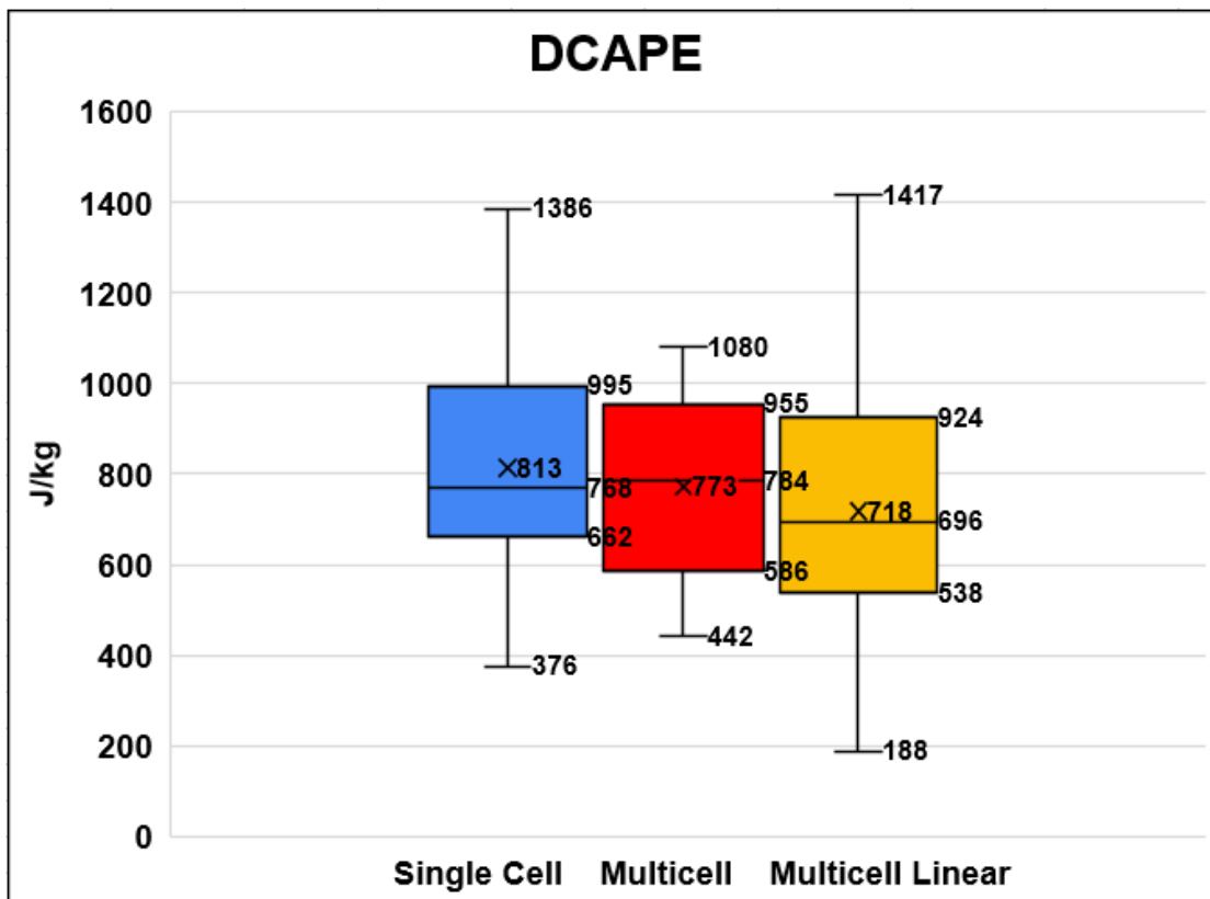
Figure 8: As in Fig. 6, except for DCAPE ( \text{J kg}^{-1} ) by storm classification type.
