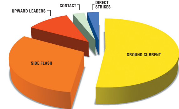
Fig 2. The frequencies of the primary lightning fatality mechanisms.
